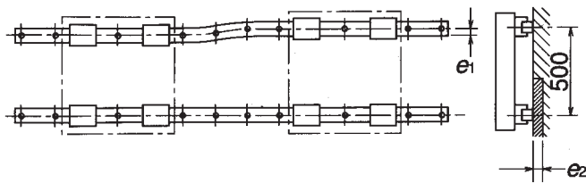
Recommended allowable installation error of the NS Series (Maximum)
