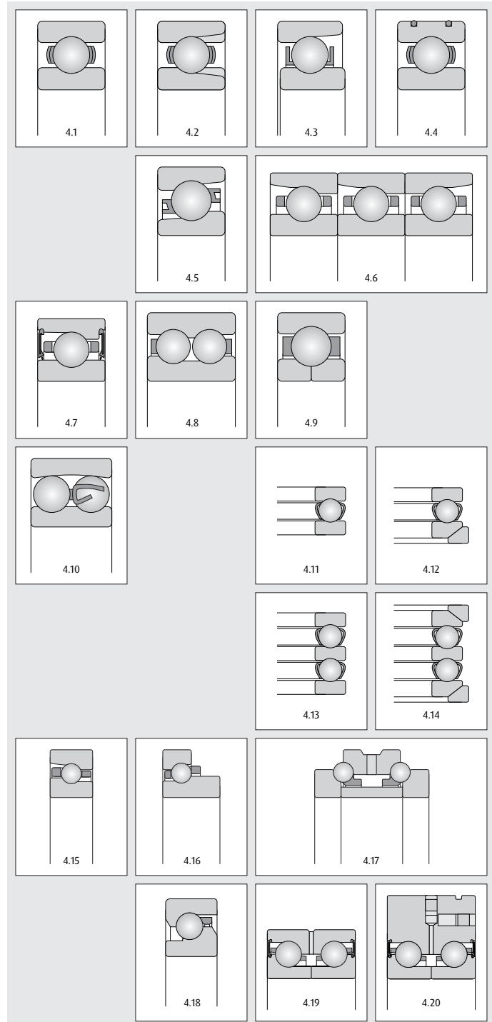
Fig. 4 - Ball Bearing Types
