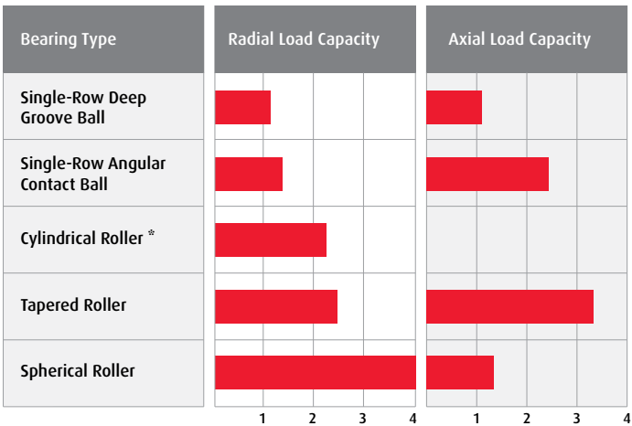
Fig. 1 - Relative Load Capacities of Bearing Types
