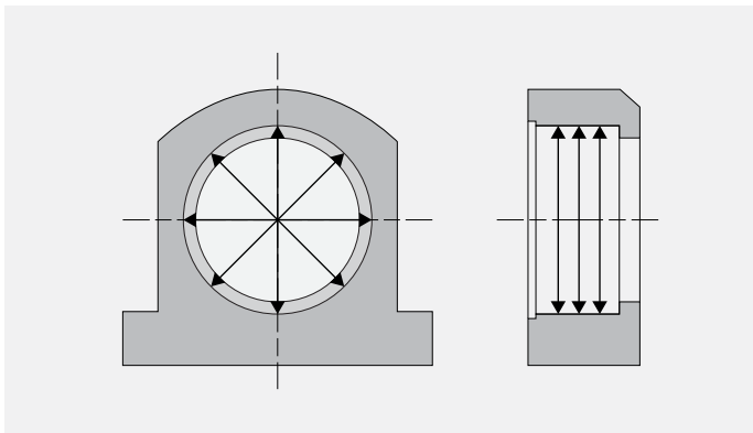
Fig. 34 - Checking Housings, Integrated Type
