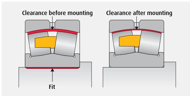
Fig. 2 - Fitting and Clearance Reduction
