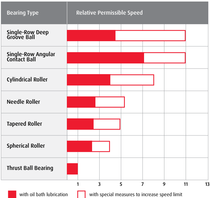
Fig. 2 - Relative Permissible Speeds of Bearing Types
