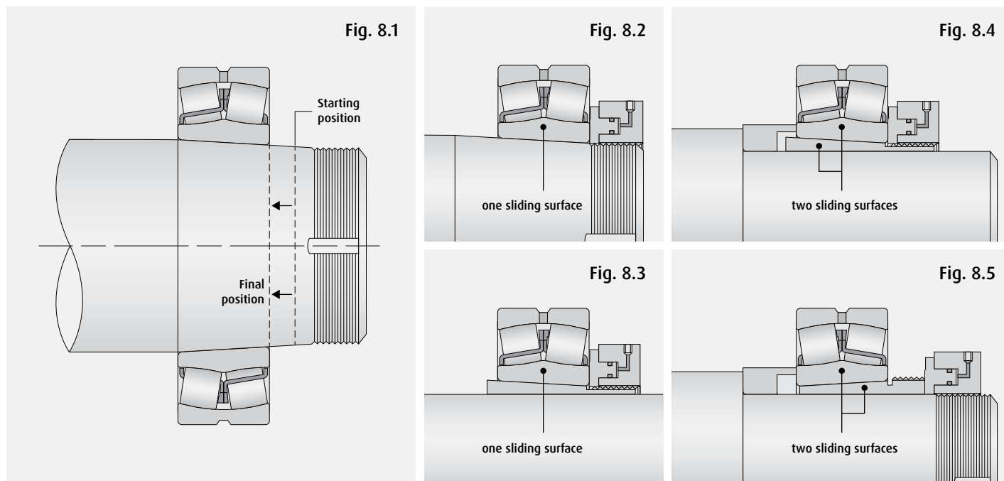
Fig. 8 - Axial Drive-Up and Sliding Surfaces
