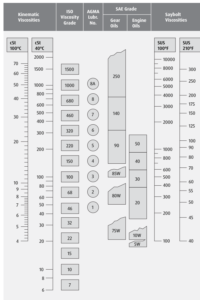
Fig. 5 - Comparative Viscosity Classifications
