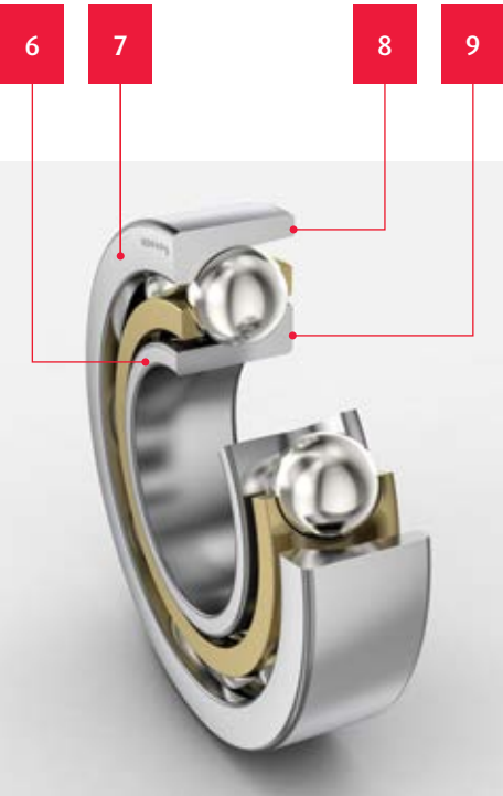
Angular contact ball bearing, single row
