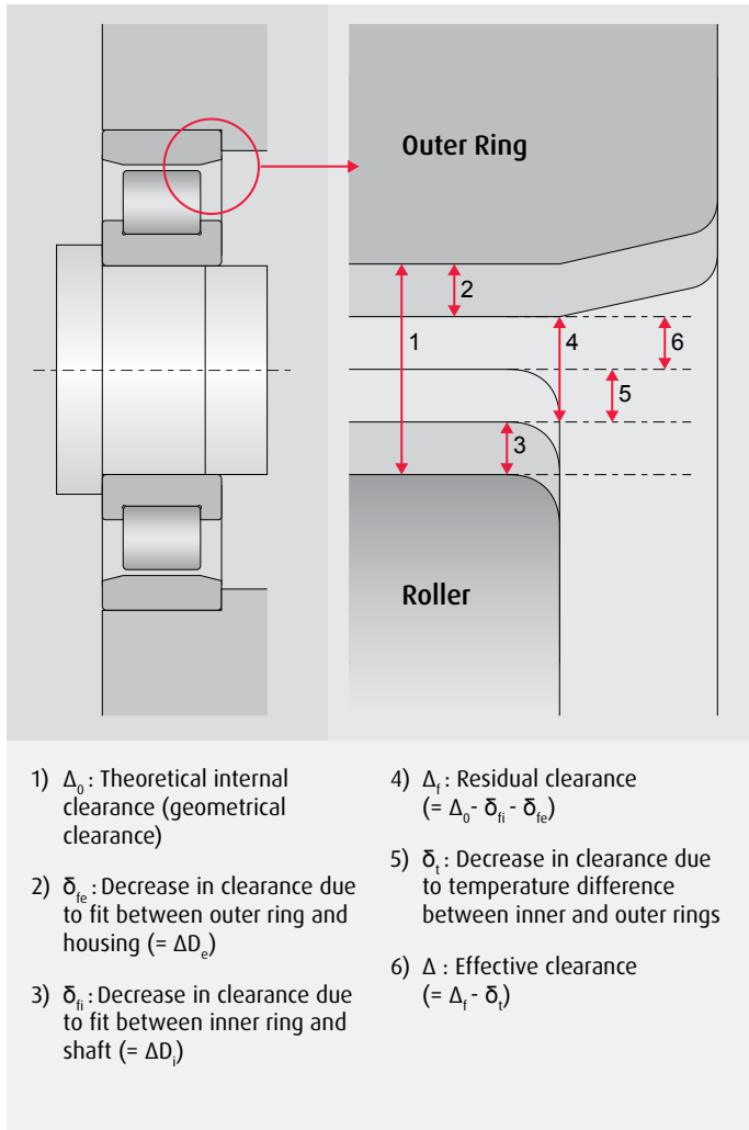
Fig. 3 - Changes in Radial Clearance of Bearings
