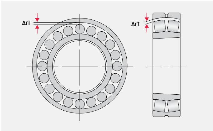
Fig. 6 - Measuring Clearance (O.D > 200 mm)
