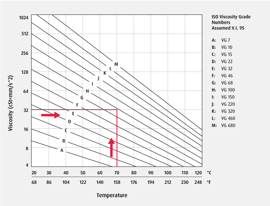
Fig. 7 - Estimate of Required Viscosity at Operating Speed
