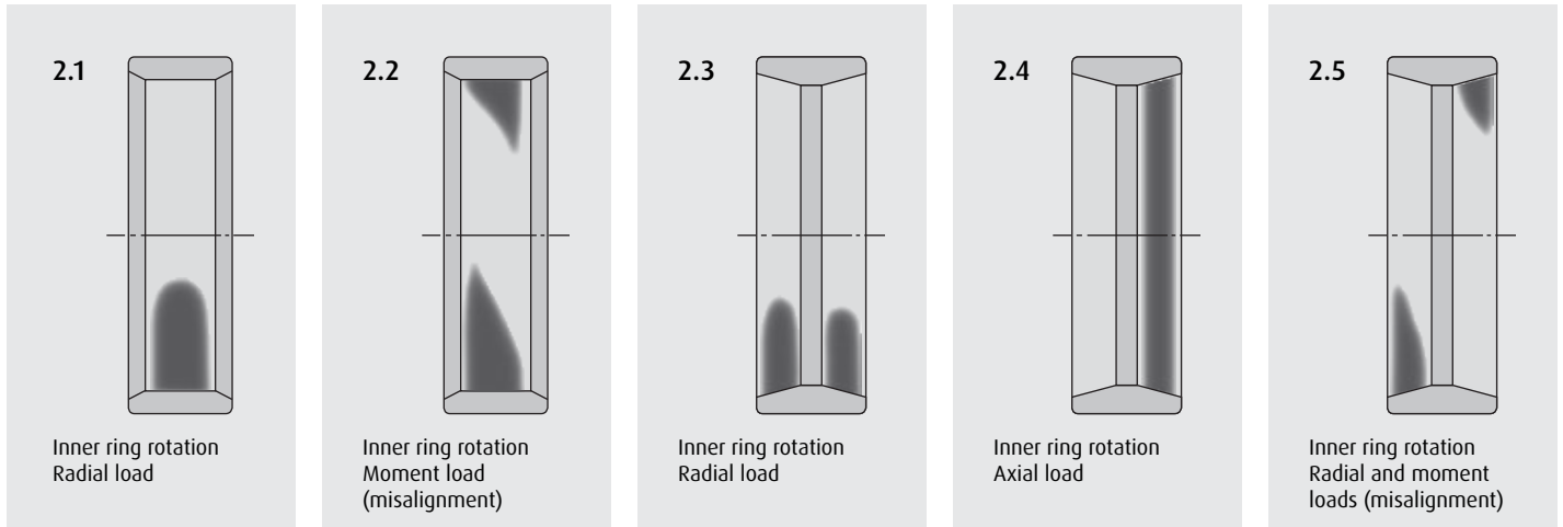
Fig. 2 - Typical Running Traces Of Roller Bearings
