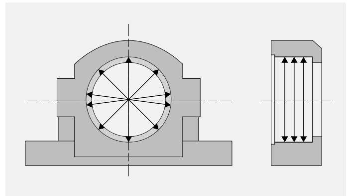
Fig. 35 - Checking Housings, Split Type
