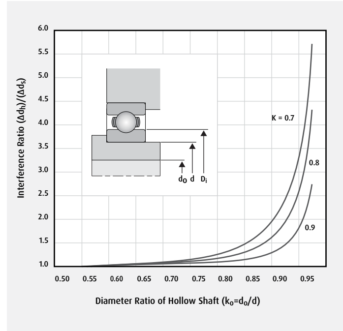
Fig. 4 - Shaft Fit Compensation for Hollow Shafts
