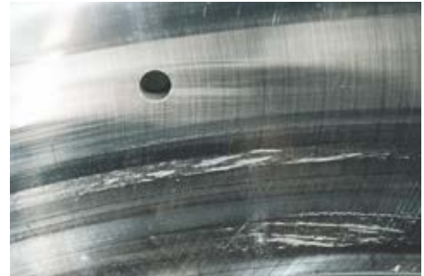
Part: Outer ring of Photo 5.5
