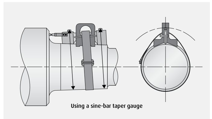
Fig. 33 - Checking Tapered Shafts
