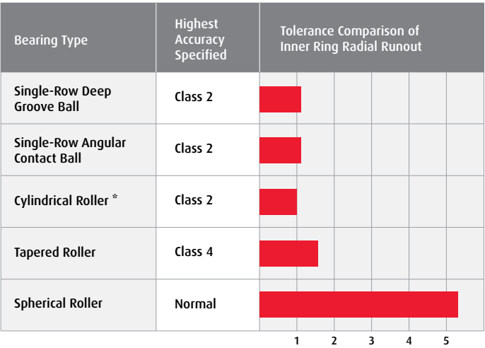
Fig. 3 - Relative Inner Ring Radial Runout of Highest Accuracy Class of Bearing Types
