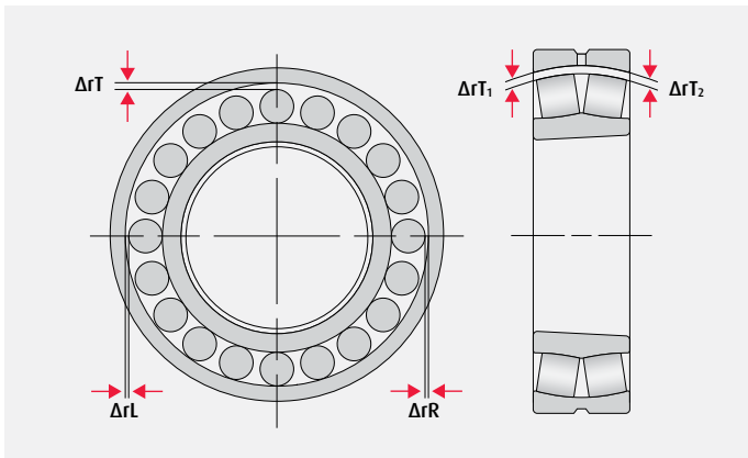
Fig. 7 - Measuring Mounted Clearance (O.D > 200 mm)
