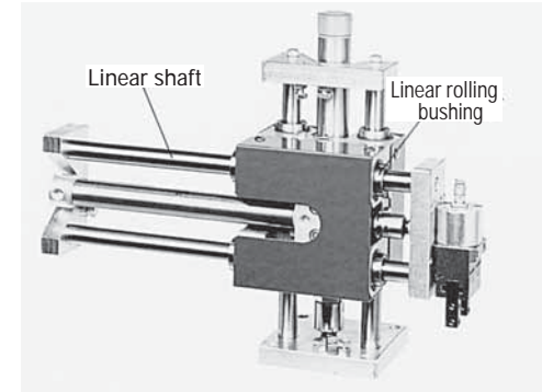
Fig. 8 Installation example
