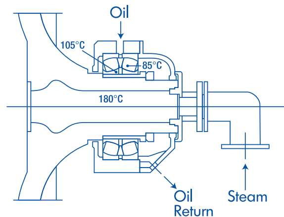
TL Application - Dryer Cylinder
