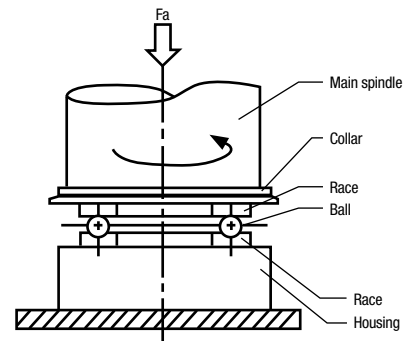
FIGURE 3 | Spindle Section of the Thrust Bearing Test Machine
