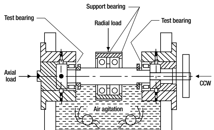
FIGURE 4 | Test Rig for Bearings Using Contaminated Lubrication
